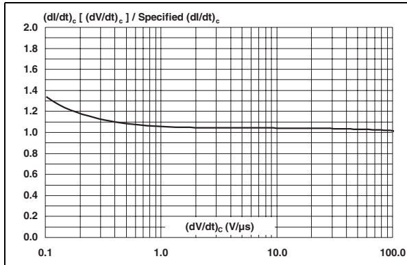
Figure 9. Relative variation of critical rate of decrease of main current (dl/dt) c versus reappplied (dV/dt) c (typical values)
